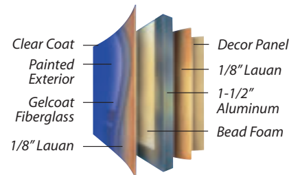
Sidewall Construction with Exterior Fiberglass
